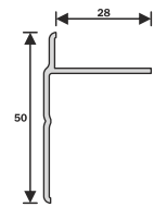
Pro40 - Everest T pervaz T Cornice profile
