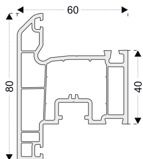
PRO521 Outward Sash Profile
