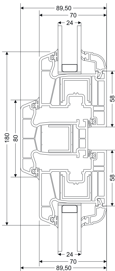
Sash - Mullion - Sash Connection Section
