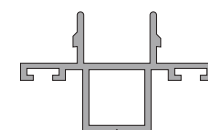
PRO411 Sliding Sash Profile Locking Plate (Alum.)
