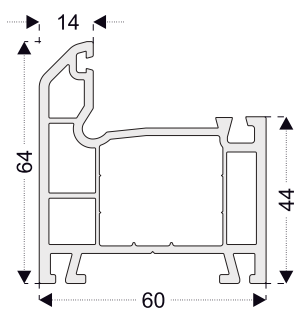
PRO51 Frame Profile
