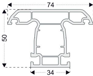
PRO533 Mullion Profile
