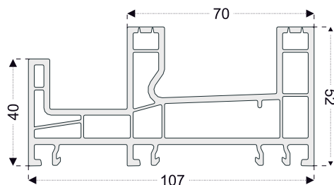
PRO232 Sliding Frame Profile with Flynet
