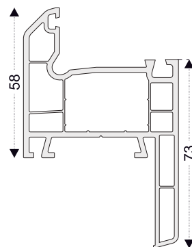
PRO81 Renovation Frame Prf.
