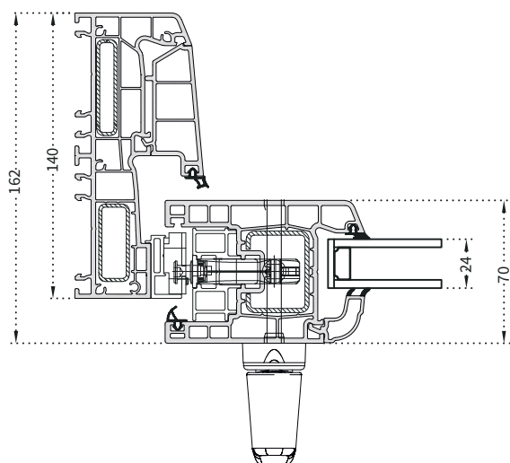
Closed Position
