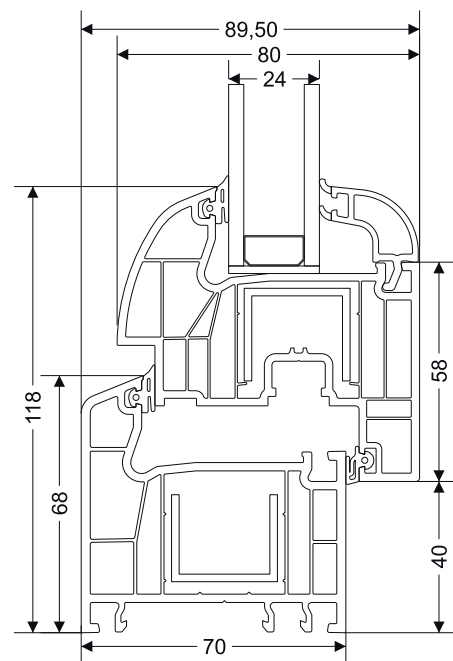
Frame - Drain Sash Connection Section
