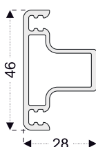
PRO235 Flynet Mullion Profile
