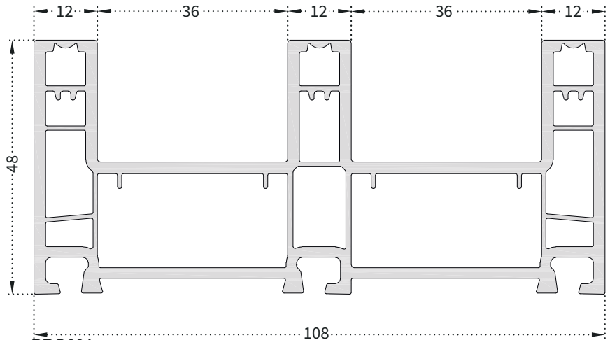
PRO601 60mm Triple Sliding Frame
