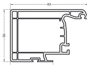
PRO215 70mm Fixed Sliding Mullion
