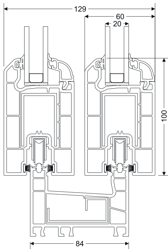
Sliding Frame - Sliding Sash 100mm
