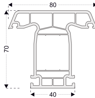
PRO713 Mullion Profile
