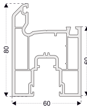
PRO21 Sliding Door Sash Profile
