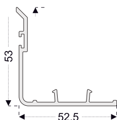
PRO214 ** for PRO213 Sliding Sash Profile Adapter
