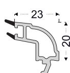
PRO703 36 mm Double Glass Glazing Bead
