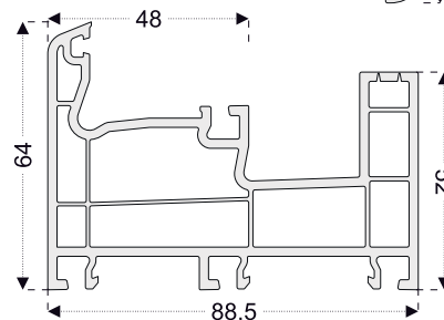
PRO231 Fixed Sliding Frame Profile
