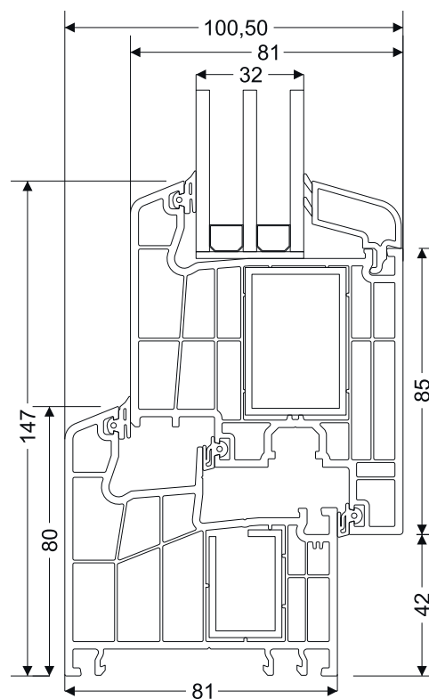
Frame - Inward Opening Door Sash Connection Section
