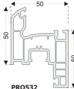
PRO532 Sash Profile
