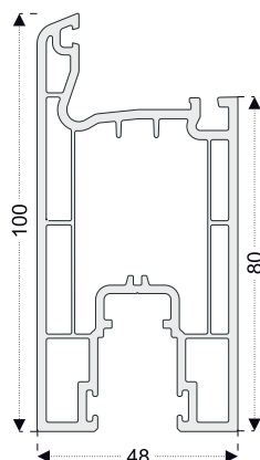
PRO213 Sliding Door Sash Profile
