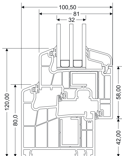
Frame - Sash Connection Section
