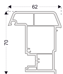
PRO717 French Casement Mullion Prf.
