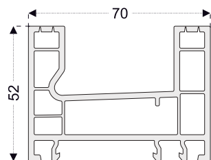
PRO201 Sliding Frame Profile
