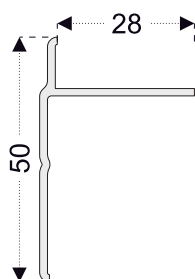
PRO35 T Trim Profile (60mm Series)
