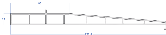
PRO75 Window Sill Profile
