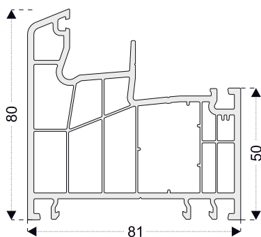
PRO8601 Frame Profile
