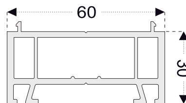
PRO14 Rising Profile - 30mm (60mm Series)
