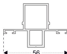
PRO41 Sliding Sash Profile Locking Plate (Alum.)
