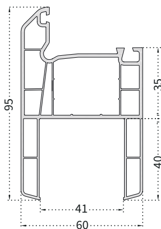
PRO15 6004 Container Frame Profile
