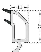
PRO07 60mm SÜRME / SLIDING 12mm Glazing Bead
