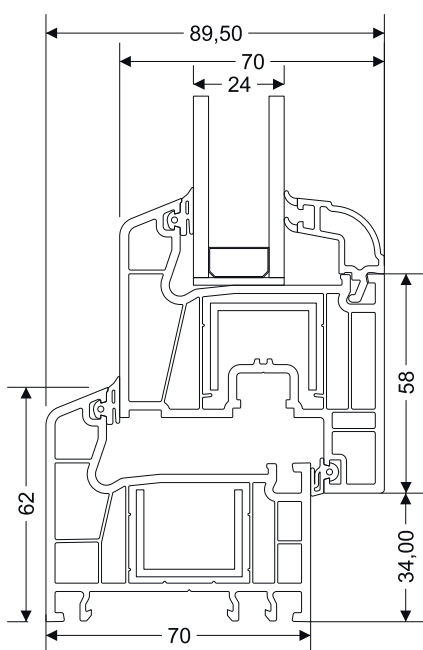
Frame 42mm - Sash Connection Section
