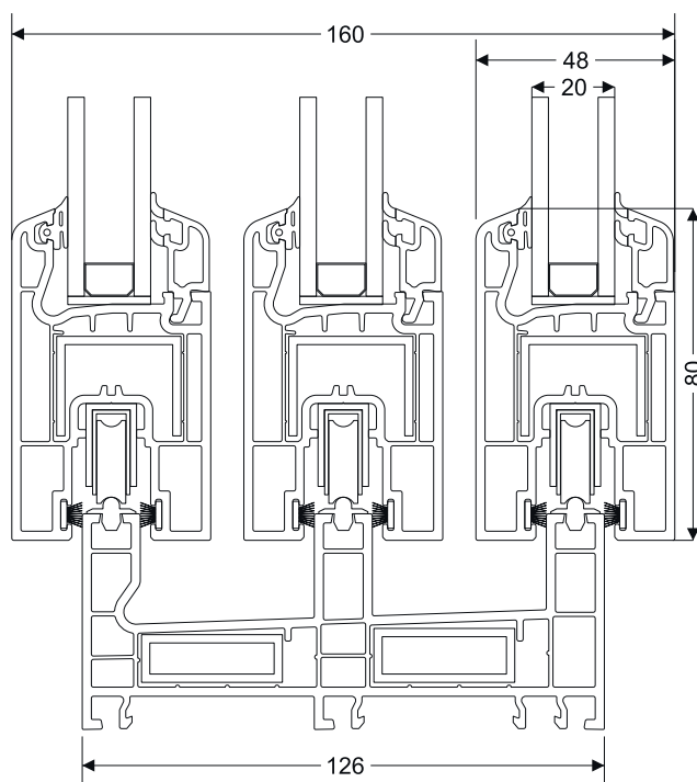
Triple Sliding Frame - Sliding Sash
