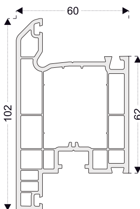
PRO10 Outward Door Profile
