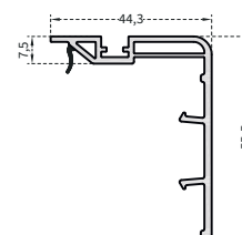
PRO216 70mm Fixed Sliding Mullion Adapter
