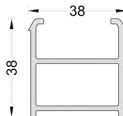
PRO1007 Hidding Rising Profile
