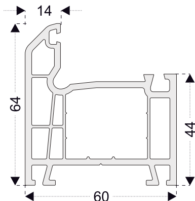
PRO01 Frame Profile
