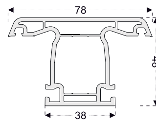
PRO212 Mullion Profile
