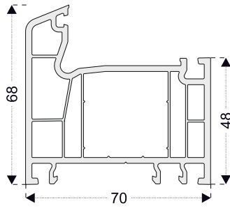
PRO710 Frame Profile - 48mm
