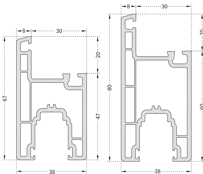
PRO604 60mm Sliding Sash (67 Mm)
