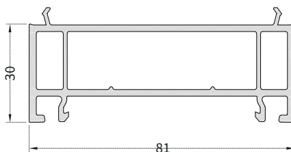
PRO8639 81mm Rising Profile
