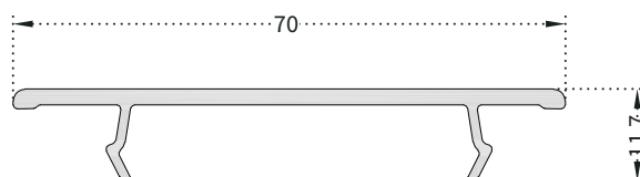
PRO1403 Sliding Sash Profile Adapter
