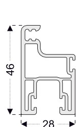
PRO234 Sliding Flynet Sash Profile
