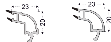
PRO702 24-26 mm Double Glass G.Bead
