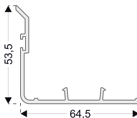
PRO25 ** for PRO24 Sliding Sash Profile Adapter
