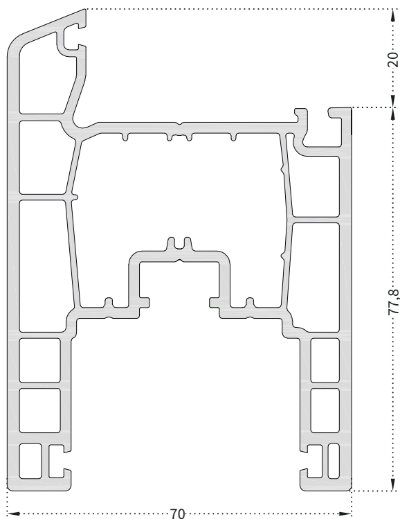
PRO1401 Sliding Sash
