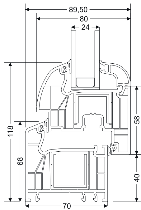
PRO7006 Frame (6 Chambers) - Drain Sash Connection Section
