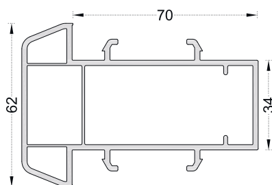
PRO37 Grillage Profile
