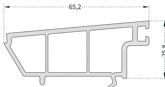
PRO1402 Sliding frame closing profile
