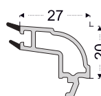
PRO700 4-6 mm Single Glass G.Bead
