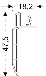
PRO38 Nailed Trim Profile (60mm Series)
