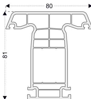
PRO8623 Mullion Profile
