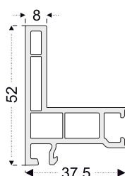
PRO205 Flynet Rail Profile
