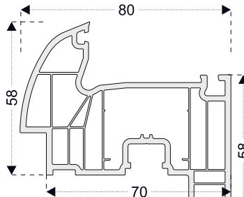
PRO724 Drain Sash Profile (7 Chambers)
