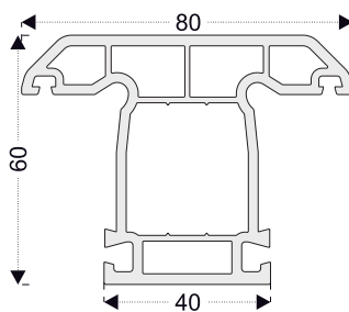
PRO53 Mullion Profile
