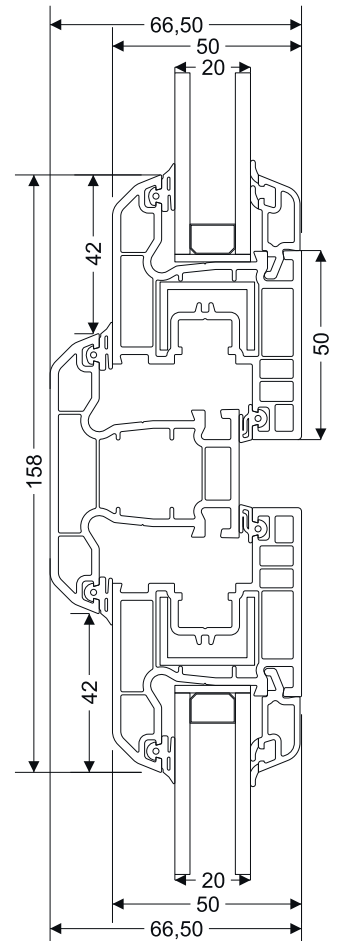
Sash - Mullion - Sash Connection Section
