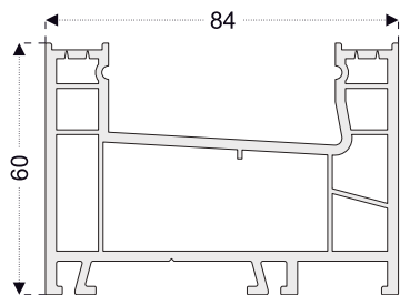
PRO20 Sliding Frame Profile
