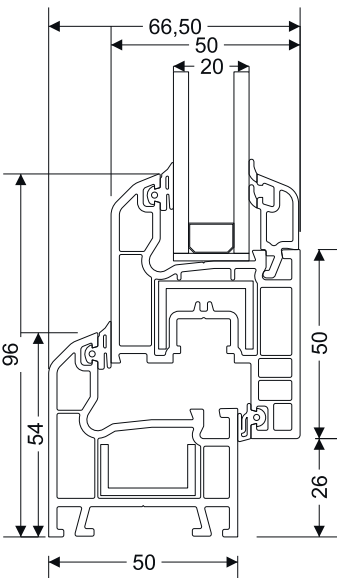
Frame - Sash Connection Section
