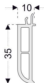
PRO39 Extension Trim Profile (70mm Series)
