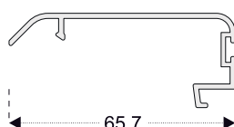
PRO43 Fixed Sliding Frame Trim Profile (Alum.)
