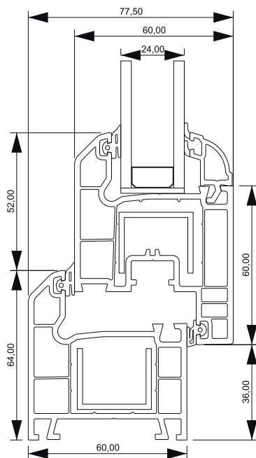
Frame - Sash Connection Section
