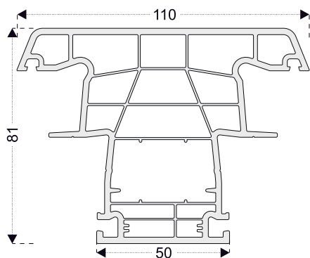
PRO8621 Mullion Profile
