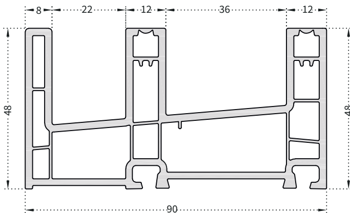
PRO602 60mm Sliding Frame With Flynet (Flynet Outside)
