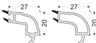
PRO701 4-6 mm Single Glass Glazing Bead
