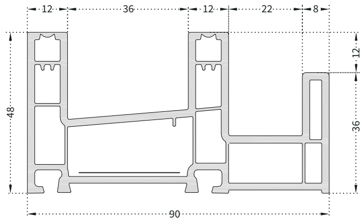
PRO603 60mm Sliding Frame With Flynet (Flynet Inside)
