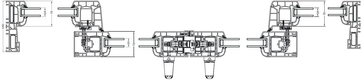
Double Sash Closed Position
