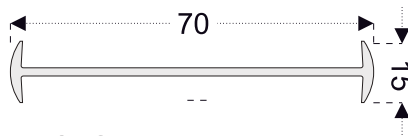
PRO79 Coupling Profile - 70mm
