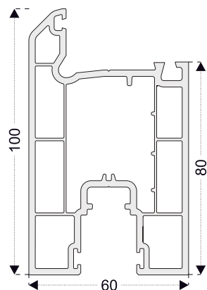
PRO24 Sliding Door Sash Profile
