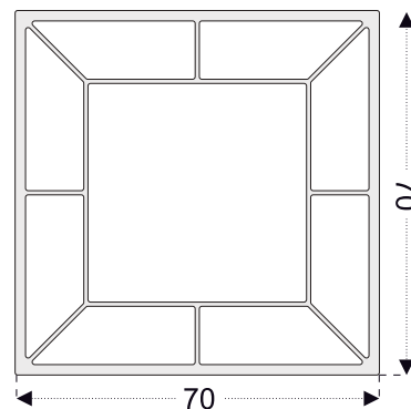
PRO80 Box Profile - 70x70mm (70mm Series)
