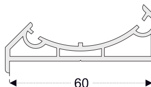
PRO33 Corner Profile - 60mm
