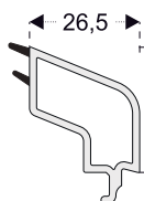
PRO8643 32mm Triple Glass Glazing Bead for Frame and Mullion Profiles PRO8601, PRO8621
