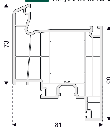
PRO8631 Inward Opening Door Profile
