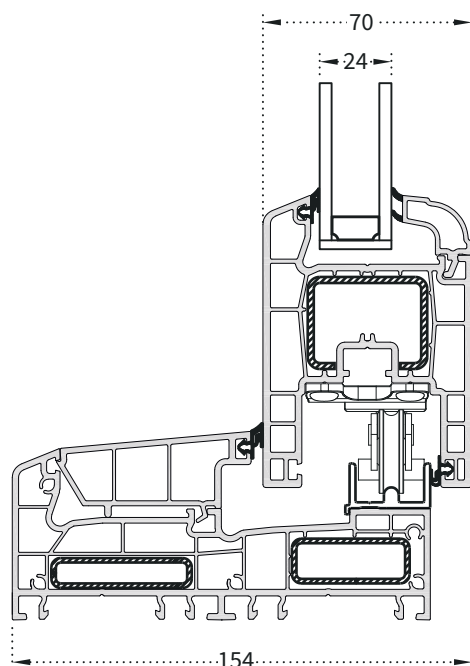
Closed Position
