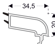
PRO8642 24mm Double Glass Glazing Bead for Sash Profiles PRO8611, PRO8631
