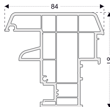
PRO8622 French Casement Mullion Profile
