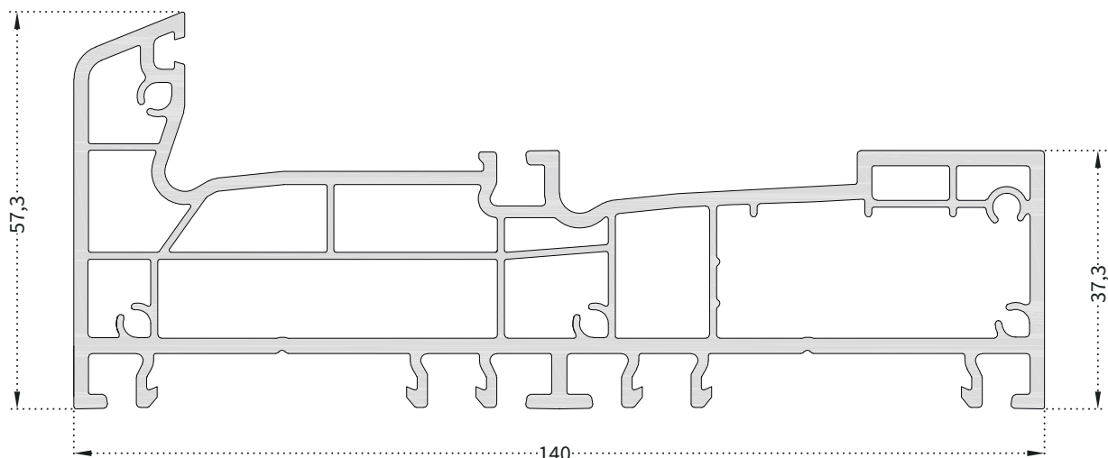
PRO1400 Sliding Frame
