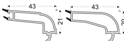
PRO700 4-6 mm Single Glass G.Bead
