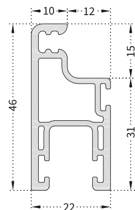
PRO607 60mm Sliding Flynet Sash
