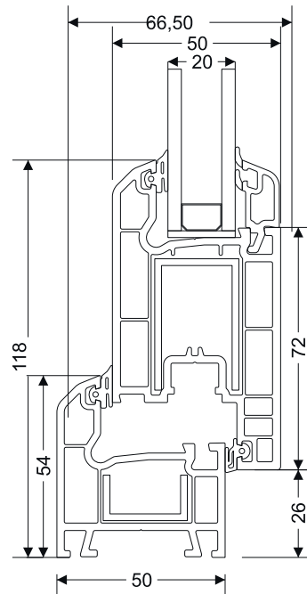
Frame - Inward Opening Door Sash Connection Section
