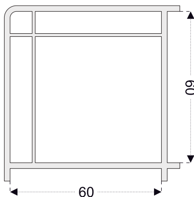
PRO36 Box Profile - 60x60mm (60mm Series)
