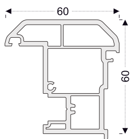
PRO12 French Casement Mullion Prf.
