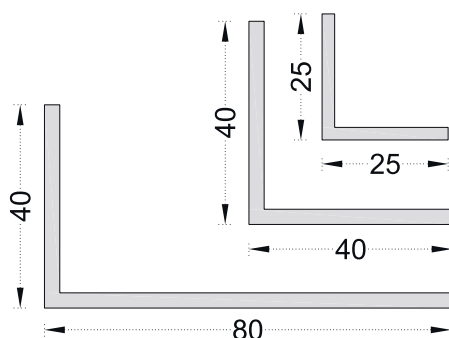
PRO1004 25x25 Corner Profile
