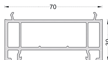
PRO1008 70mm Rising Profile
