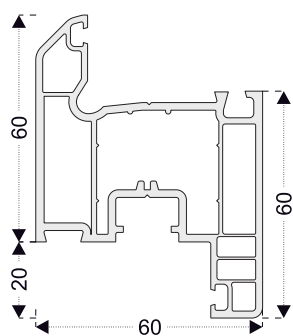
PRO52 Sash Profile
