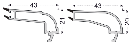
PRO700 4-6 mm Single Glass G.Bead
