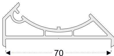
PRO331 Corner Profile - 70mm
