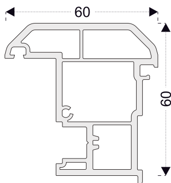
PRO12 French Casement Mullion Prf.
