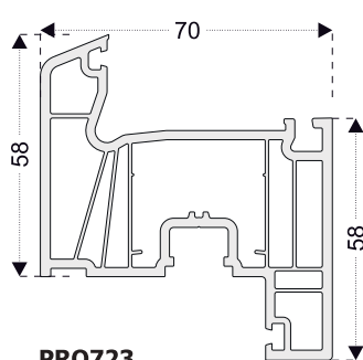
PRO723 Sash Profile (6 Chambers)
