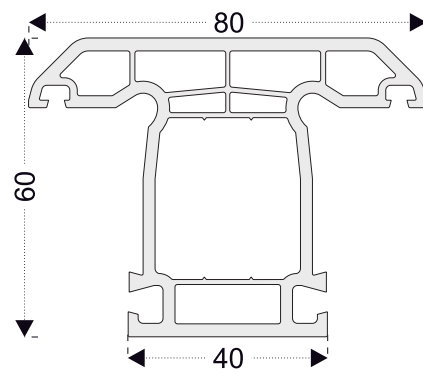
PRO03 Mullion Profile
