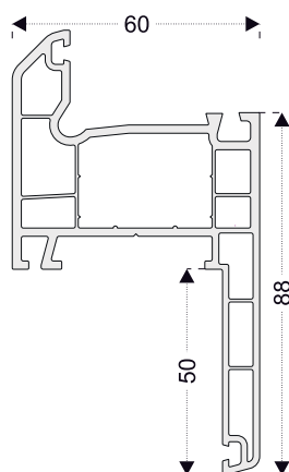
PRO82 Renovation Frame Prf.
