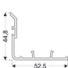
PRO204 ** for PRO211 Sliding Sash Profile Adapter
