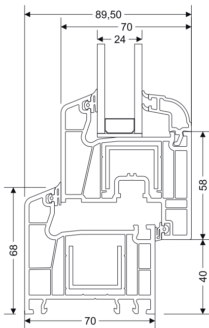
Frame 48mm - Sash Connection Section
