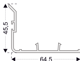
PRO22 ** for PRO21 Sliding Sash Profile Adapter
