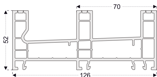
PRO2011 Triple Sliding Frame Profile
