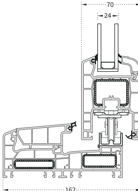
Sliding Position
