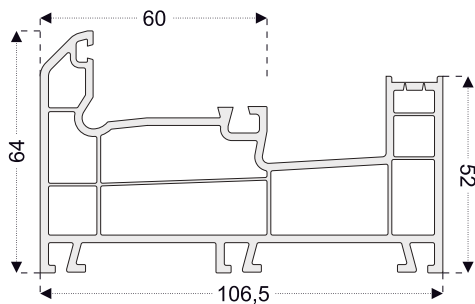
PRO23 Fixed Sliding Frame Profile
