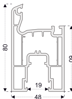
PRO211 Sliding Door Sash Profile
