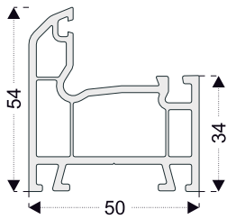
PRO531 Frame Profile
