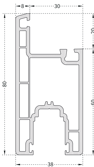
PRO605 60mm Sliding Sash (80 Mm)
