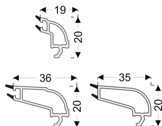
PRO05 20-22 mm Double Glass G.Bead
