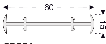
PRO34 Coupling Profile - 60mm
