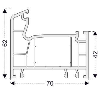
PRO711 Frame Profile - 42mm
