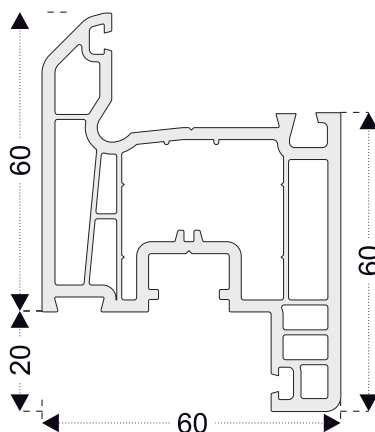
PRO02 Sash Profile
