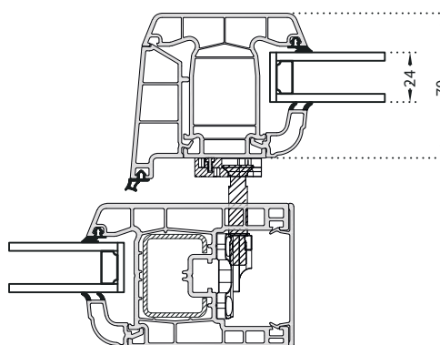
Sliding Position
