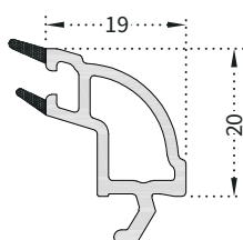
PRO05 60mm SÜRME / SLIDING 4mm Glazing Bead
