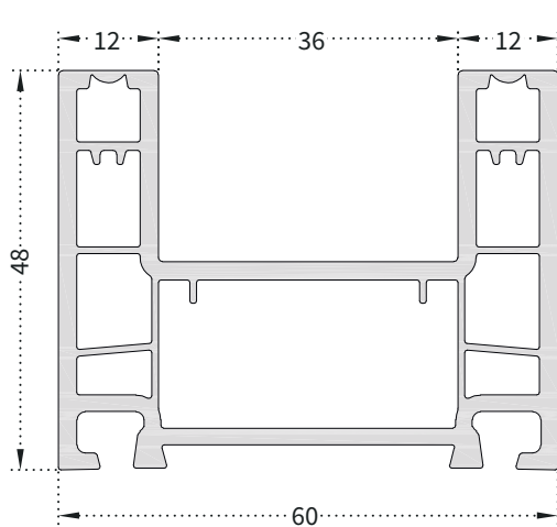
PRO600 60mm Sliding Frame
