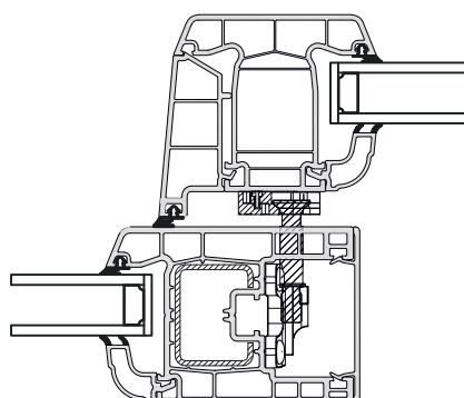
Closed Position
