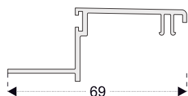
PRO28 Double Sliding Frame Trim Profile (Alum.)
