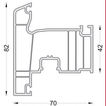
PRO722 Outward Sash
