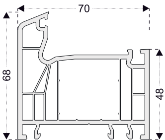
PRO720 Frame Profile (6 Chambers)
