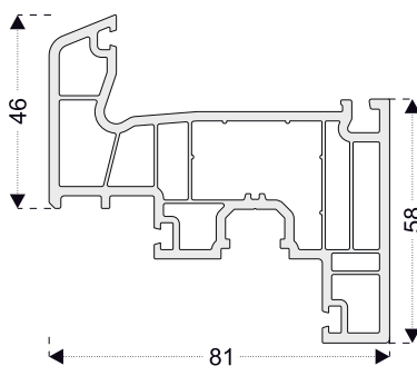
PRO8611 Sash Profile
