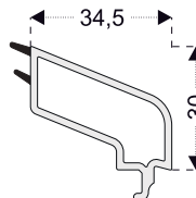
PRO8644 24mm Double Glass Glazing Bead for Frame and Mullion Profiles PRO81601, PRO8621
