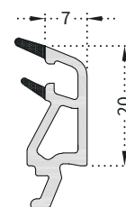
PRO704 60mm SÜRME / SLIDING 16mm Glazing Bead
