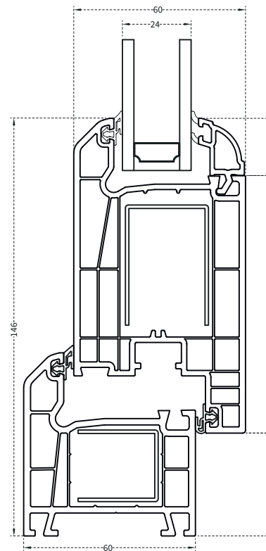
Frame - Inward Opening Door Sash Connection Section
